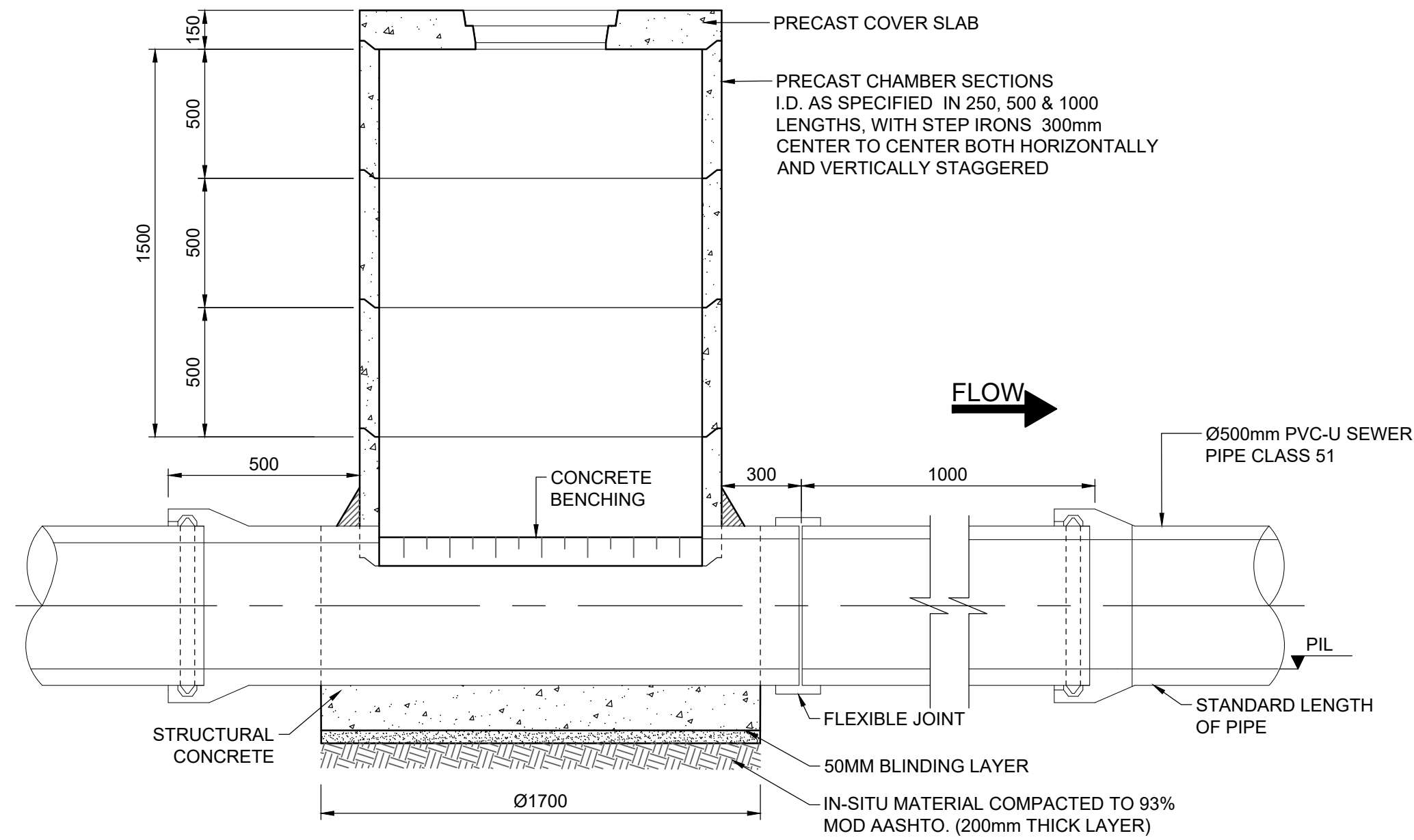
SECTION 02-02 SCALE 1:20
