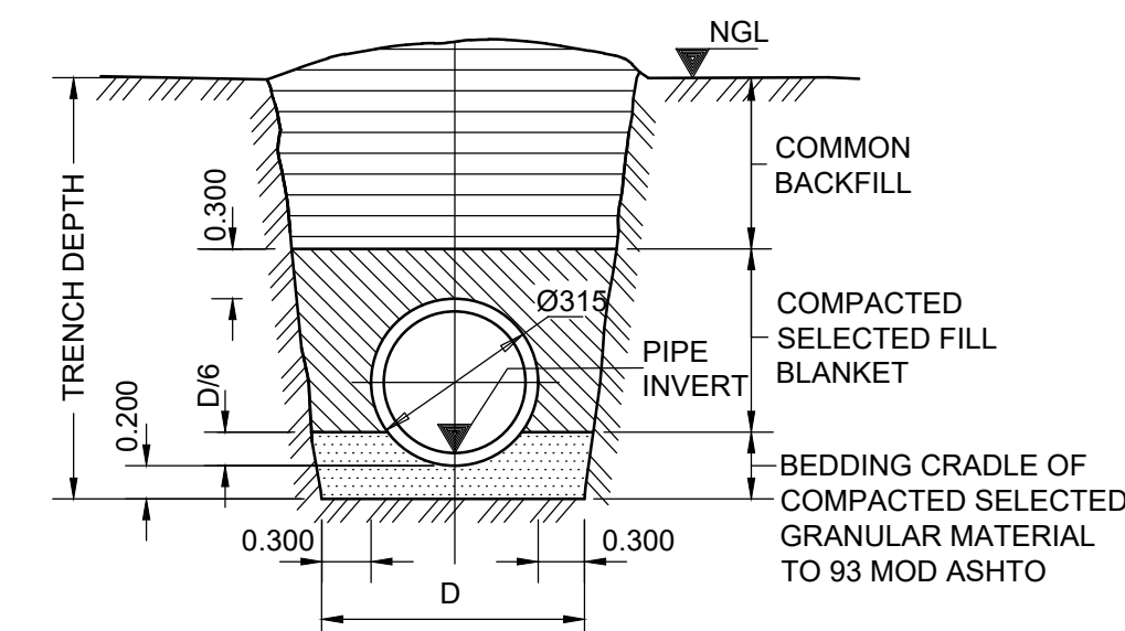
SECTION 01-01 - POSITION OF PIPELINE IN SERVITUDE STRIP N.T.S
