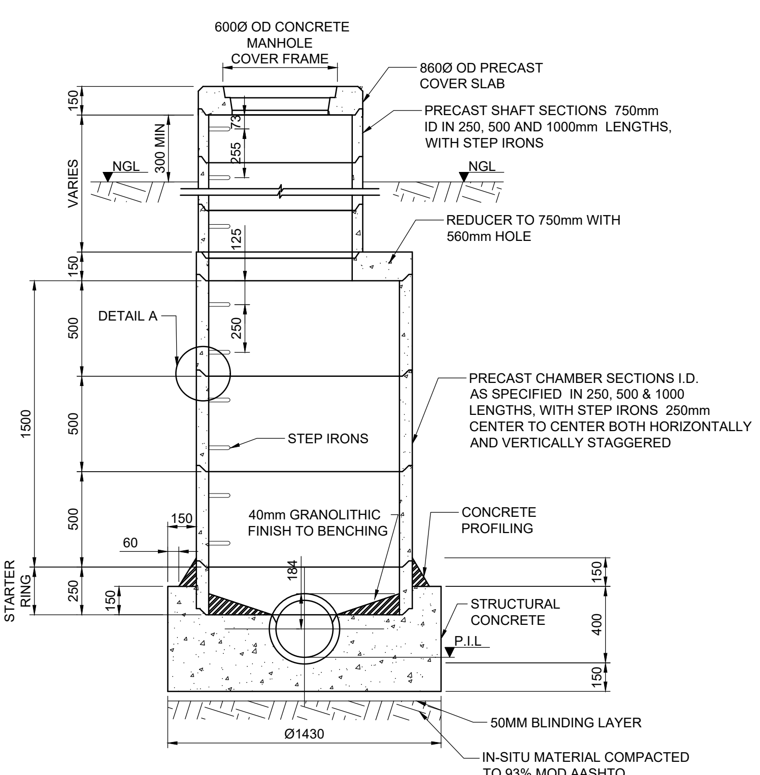
SECTION 01-01 SCALE 1:20
