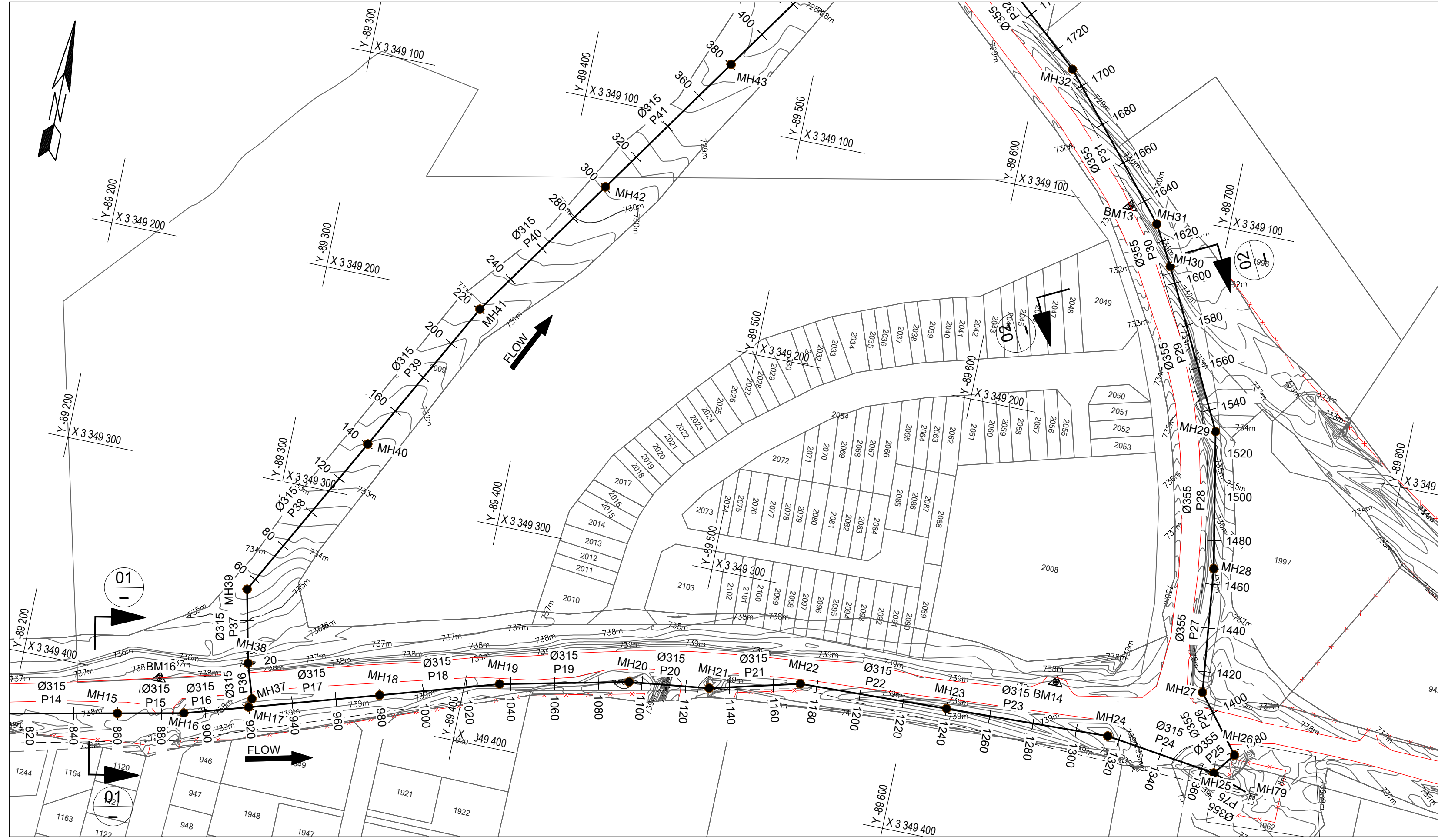
PLAN LAYOUT SCALE 1:1500
