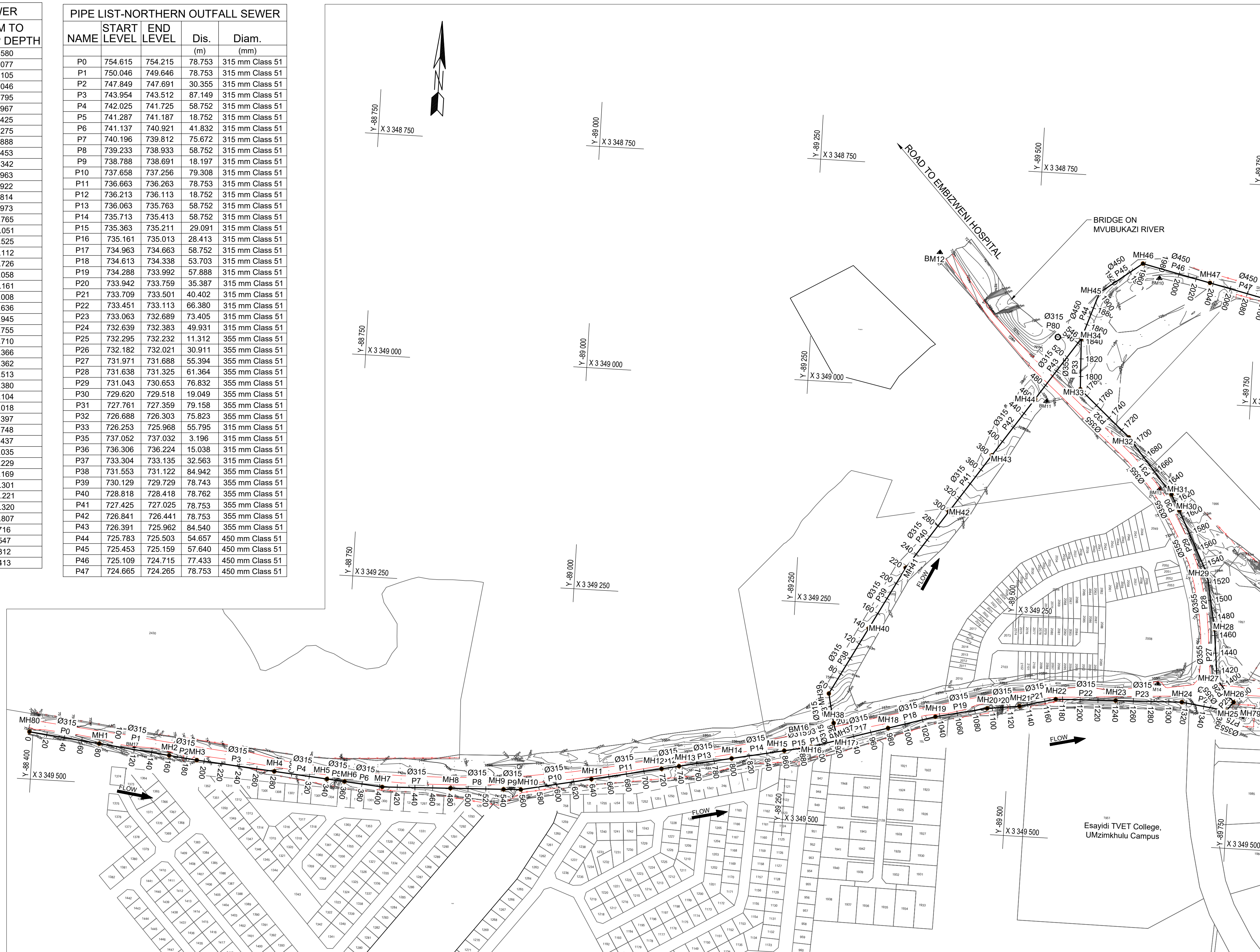
NORTHERN OUTFALL SEWER PLAN SCALE 1:2500
