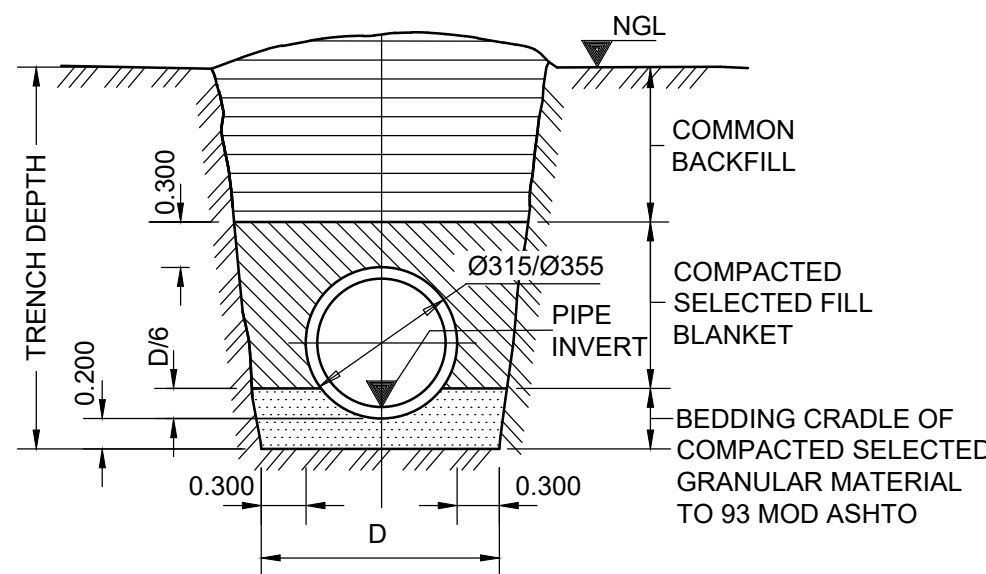
TYPICAL TRENCH CROSS-SECTION N.T.S
