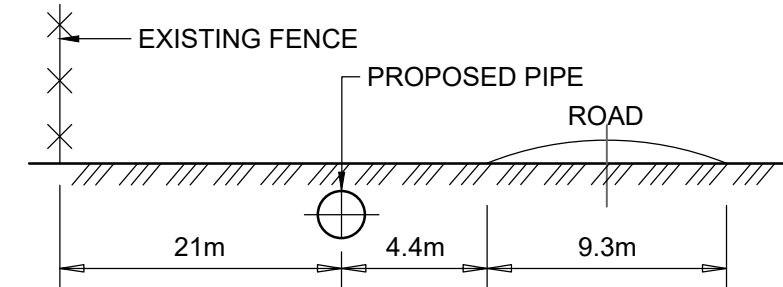
SECTION 02-02 - POSITION OF PIPELINE IN SERVITUDE STRIP N.T.S
