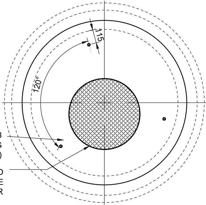
MANHOLE COVER SCALE 1:20
