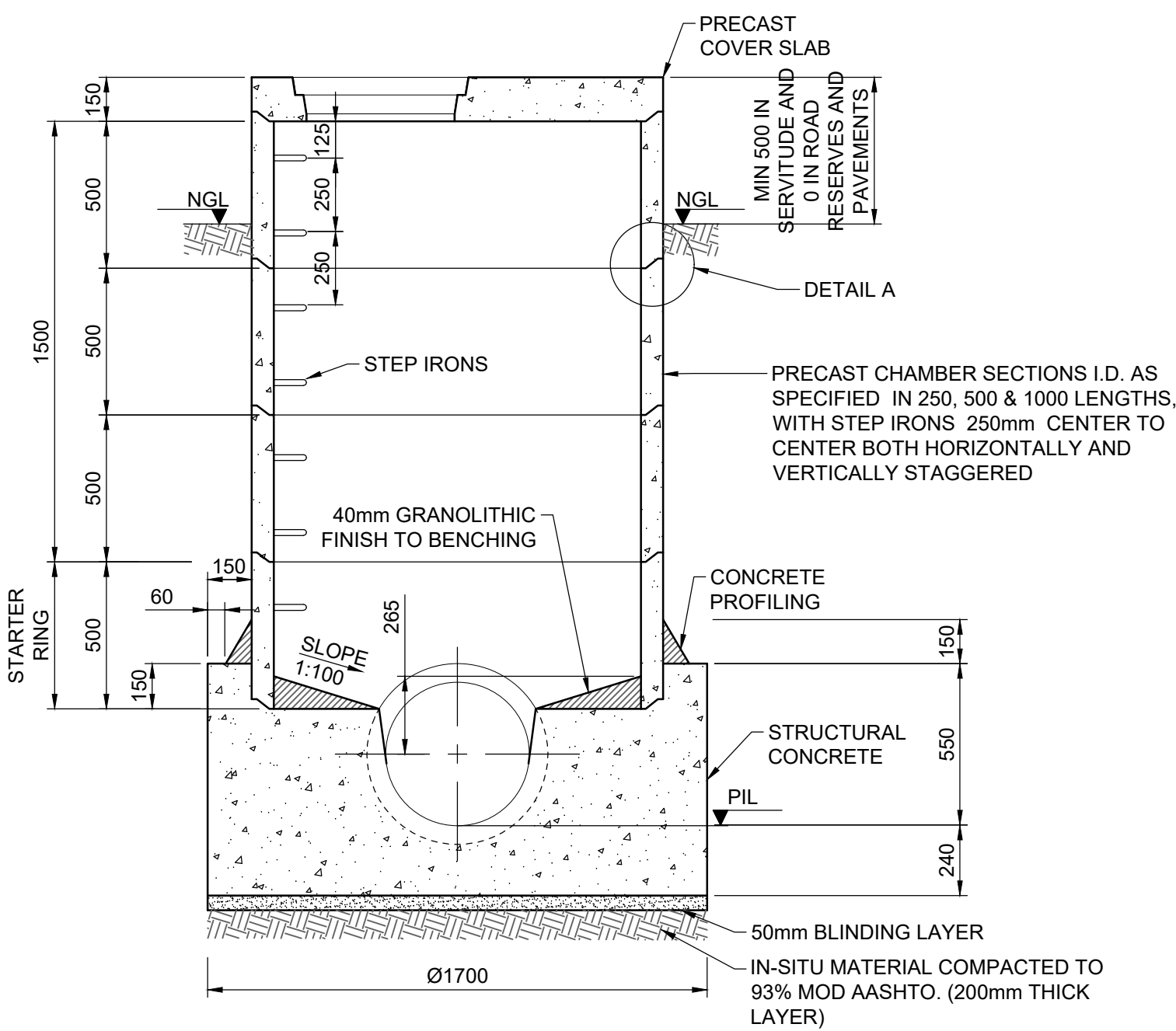
SECTION 01-01 SCALE 1:20
