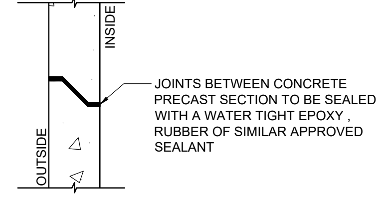
DETAIL A SCALE 1:5
