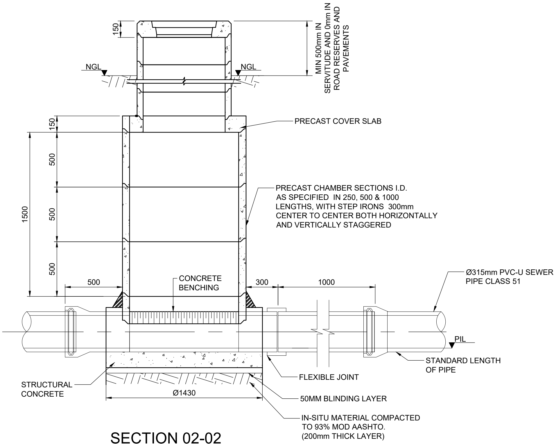
SECTION 02-02 SCALE 1:20
